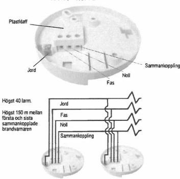
FIGUR 5 – KOPPLING
